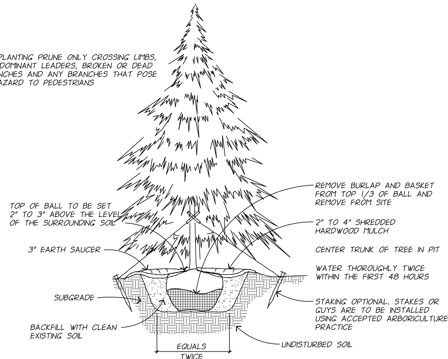
2 TYPICAL TREE PLANTING DETAIL L.I.O. NO SCALE
