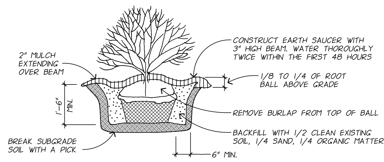
3 TYPICAL SHRUB PLANTING DETAIL L.I.O. NO SCALE
