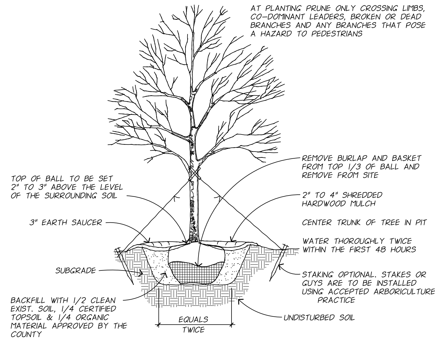
1 TYPICAL TREE PLANTING DETAIL L.I.O. NO SCALE
