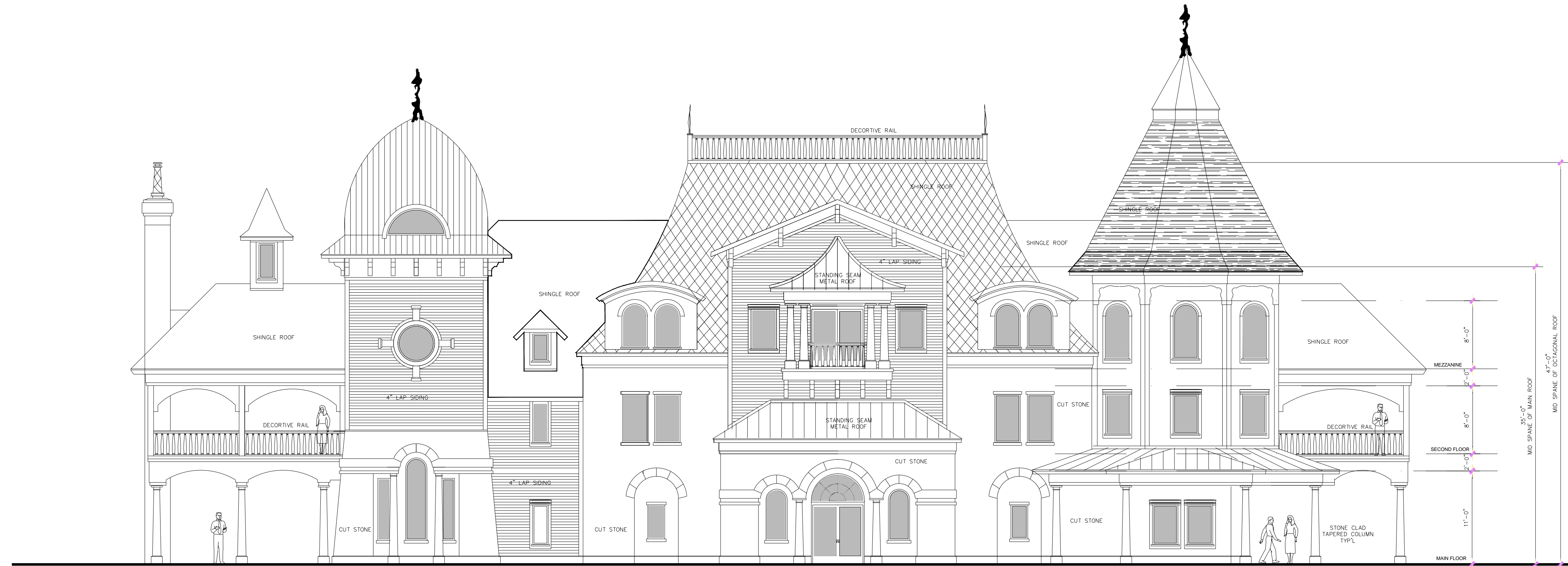
Front Building Elevation Scale: 1/8" = 1'-0"
